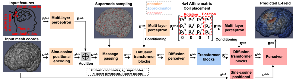
Figure 1: Schematics of the proposed transformer-based neural PDE surrogate.
