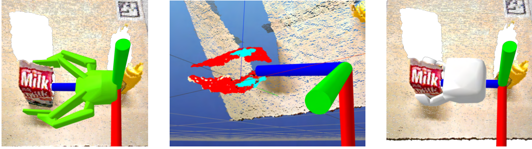
(a) Robotiq 2F-140 parallel-jaw gripper with a red 'Milk' can. (b) Width estimation using the augmented point cloud. (c) HSR gripper kinematics with an arc-shaped closing trajectory.
