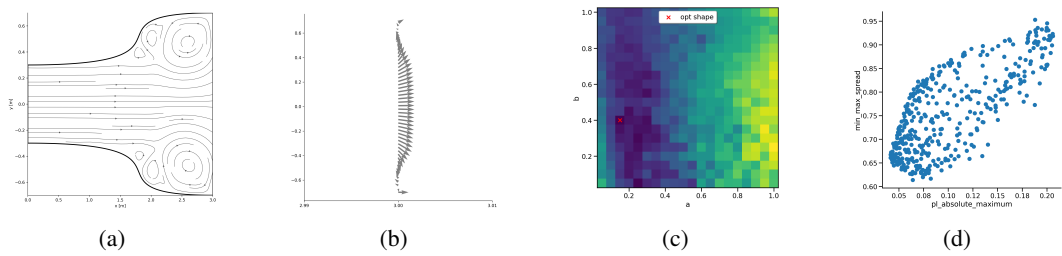
Figure 2: (a) Diffuser channel geometry and a snapshot of the velocity field for a representative shape; (b) velocity field at the diffuser outlet; (c) heatmap of the objective function over the shape search space; (d) scatter plot of the objective value versus a low-cost physical feature.
