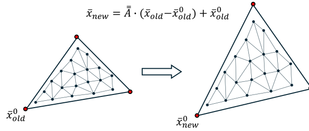
Figure 3: Mesh deformation methodology
