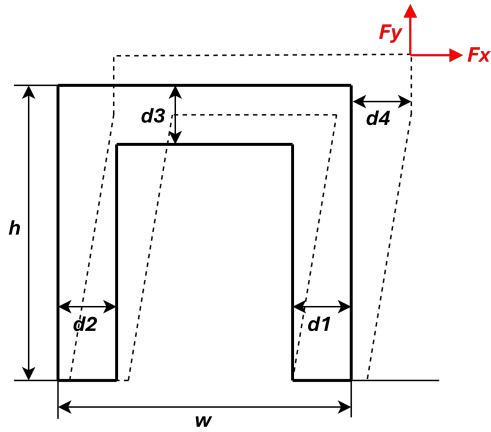
Figure 4: Illustration of the frame model with six geometric and two load parameters. The Young's modulus is E = 1000 MPa.
